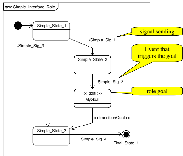
Figure 2. The state machine of a semantic interface
