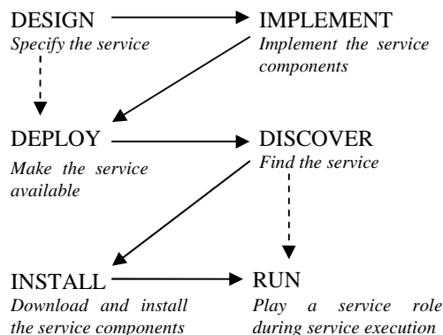
Figure 3. The SIMS service lifecycle
