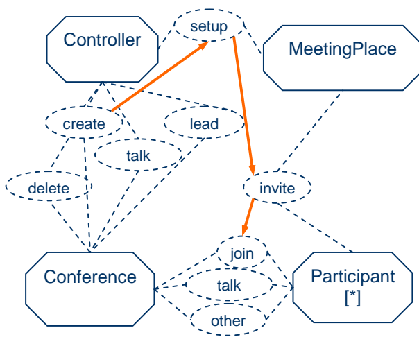
Figure 5. The design of a virtual meeting place
